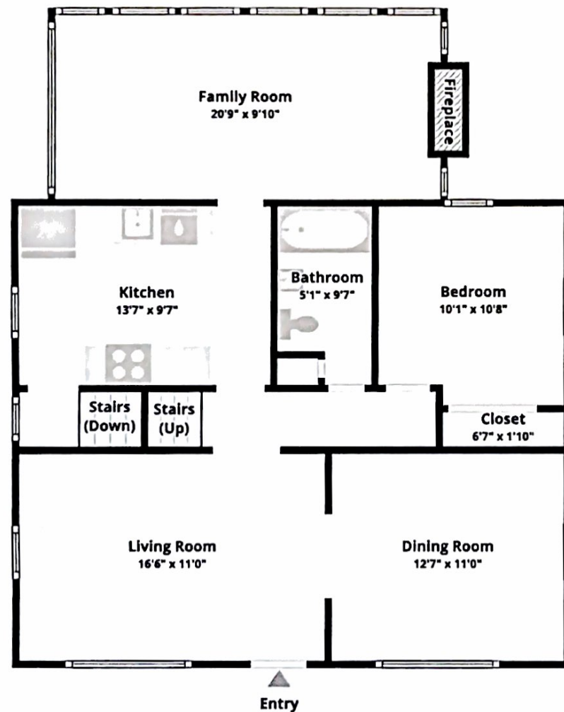
FLOOR 1
